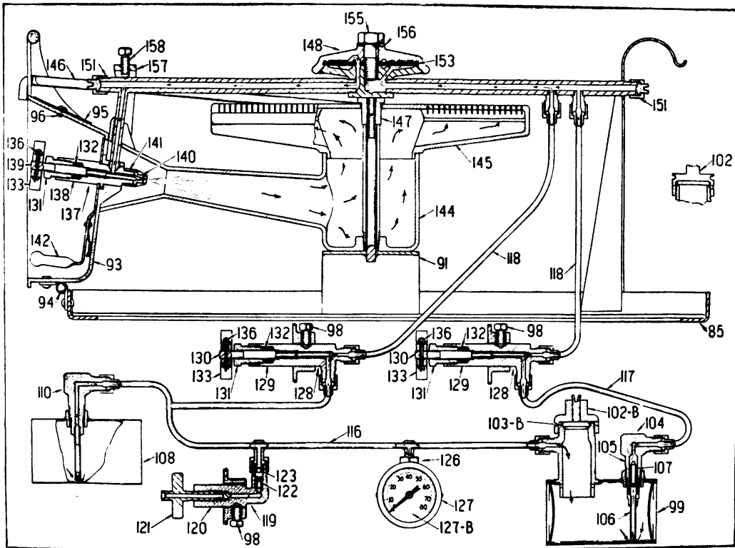
FIGURE 36.—Sectional view of gasoline fire unit.
